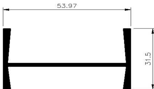
Transom/Post Section No. FPX00304 Weight 0.0687kg/m Periphery 234mm ext
