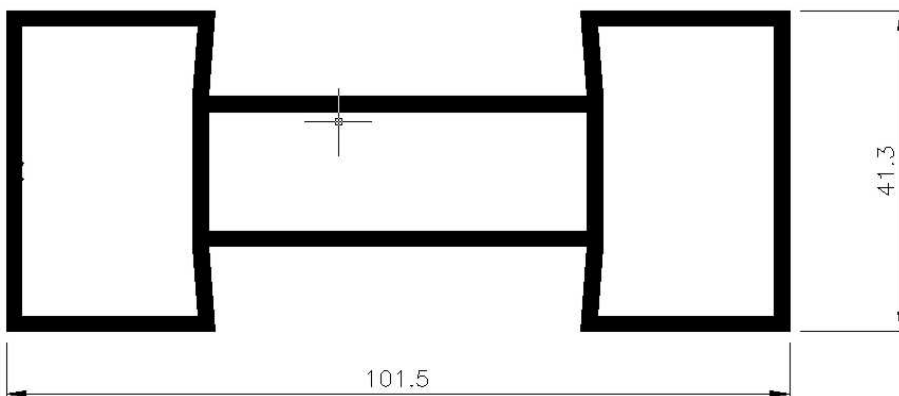
Cover Plate Section No. 54995 Weight 0.251 kg/m Periphery 118mm ext
