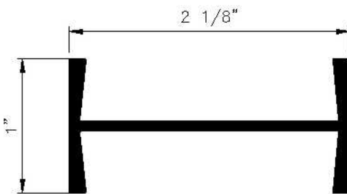
Transom/Post (Imperial) Section No. FPX00401 Weight 0.624kg/m Periphery 209mm ext
