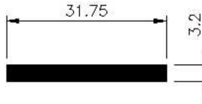
31.75 x 3.2 Flat Bar Section No. 11006 Weight 0.275 kg/m Periphery 70mm ext
