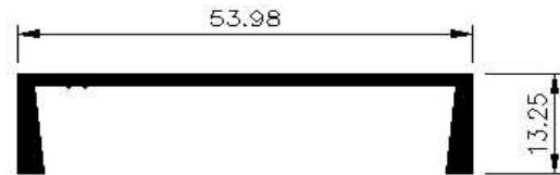
Shallow Channel Section No. 54868 Weight 0.394 kg/m Periphery 240mm ext
