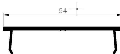
Cover Plate Section No. FPX00305 Weight 0.329 kg/m Periphery 157mm ext
