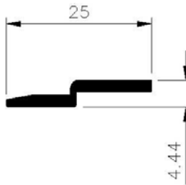
Wall Bracket Section No. FPX00338 Weight 0.142kg/m Periphery 56mm ext
