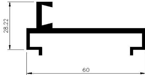
Door Frame Section No. FPX00314 Weight 0.813kg/m Periphery 240mm ext
