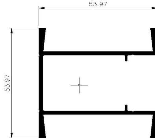
Wiring Post Section No. 53331 Weight 0.983 kg/m Periphery 380mm ext
