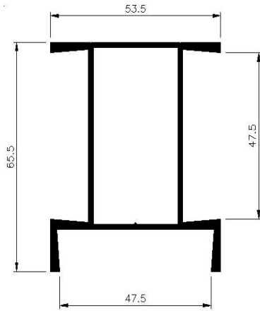
3 Way Post Section No. 19252 Weight 1.138 kg/m Periphery 317mm ext/ 154 mm int
