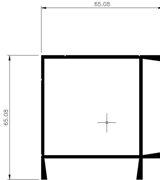
Corner Post Section No. 19251 Weight 1.192 kg/m Periphery 313mm ext/ 203 mm int
