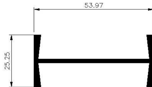
Transom/Post (metric) Section No. 53330 Weight 0.600kg/m Periphery 209mm ext
