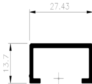
Cover Plate Section No. 54995 Weight 0.251 kg/m Periphery 118mm ext
