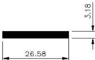
26.58 x 3.18 Flat Bar Section No. FPX00333 Weight 0.246 kg/m Periphery 64mm ext
